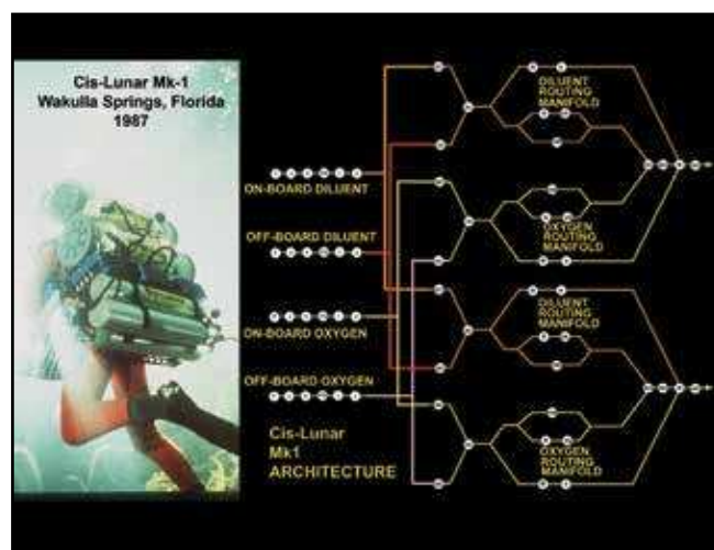
Figure 10. A fault-tree diagram for a fully redundant rebreather (at right). At left, early testing of the Cis-Lunar Mk1 redundant rebreather known as “FRED” (Failsafe Rebreather for Exploration Diving).
