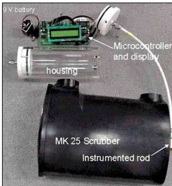
Figure 11. Photograph of the proof-of-concept unit developed for the U.S. Navy MK 25 100 percent O 2 rebreather. This unit was meant for verifications and demonstrations, not for field use.
