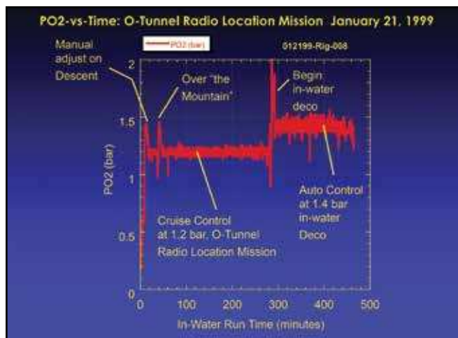
Figure 51. Typical base-level stored data from the Mk5 rebreather: \text{PO}_2 versus time.
