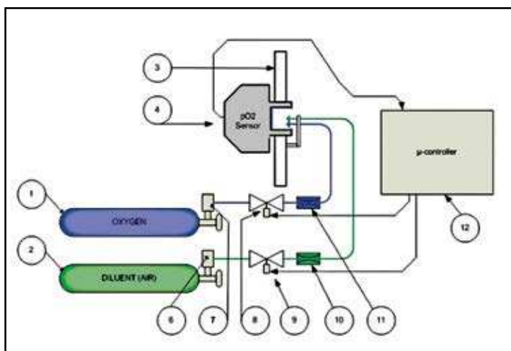
Figure 3. Schematic of our true PO 2 sensor signal validation system (1: O 2 tank; 2: diluent tank; 3: sensor support; 4: PO 2 sensor; 6, 7: pressure regulators; 8, 9: solenoids; 10, 11: flow restriction orifices; 12: microcontroller). Reprinted with permission of Diving and Hyperbaric Medicine (Sieber et al., 2008).
