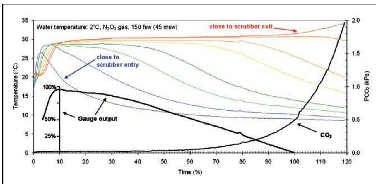
Figure 9. Temperature and CO 2 variations recorded from eight sensors placed in a CO 2 scrubber. The calculated gauge output is also shown.
