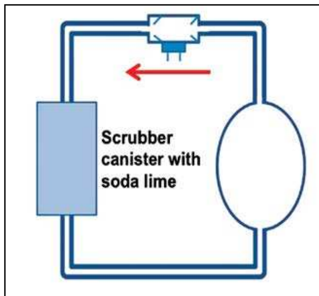
Figure 2. Simplified and stylized depiction of a basic rebreather circle circuit or "loop" with a \text{CO}_2 scrubber canister added.
