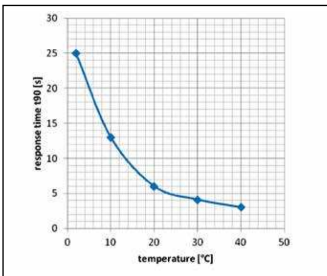
Figure 2. Response time of galvanic O_2 sensors depends on temperature.
