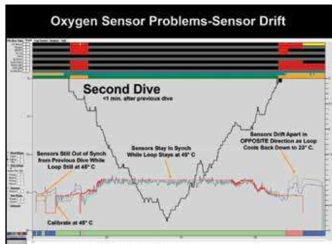
Figure 55. Recalibration of differentially heated oxygen sensors while the sensors are in use leads to stable lock, but the sensors drift apart when the dive is over (and the canister is no longer generating heat). Such behavior highlights the temperature sensitivity of the galvanic-style oxygen sensors that are used in every rebreather today. Dealing with this means tracking the precise temperature of each oxygen sensor and compensating for the temperature change in the reported PO_2 .
