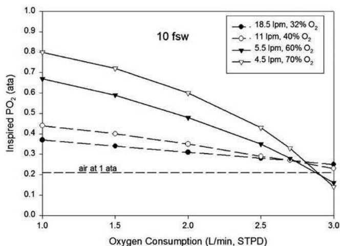
Figure 11. High flow-rate CMI rebreathers of the past were relatively insensitive to changes in diver oxygen consumption. John R. Clarke figure.
