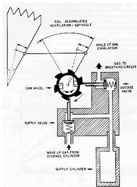
Figure 21. Interspiro ACSC ventilation control mechanism.
