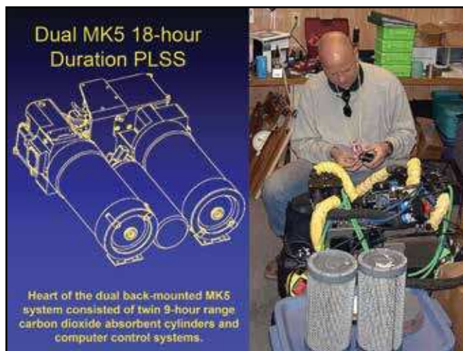
Figure 20. Assembly of the dual backmounted rebreather. The device used two radial hydrophobic carbon-dioxide absorbent canisters.
