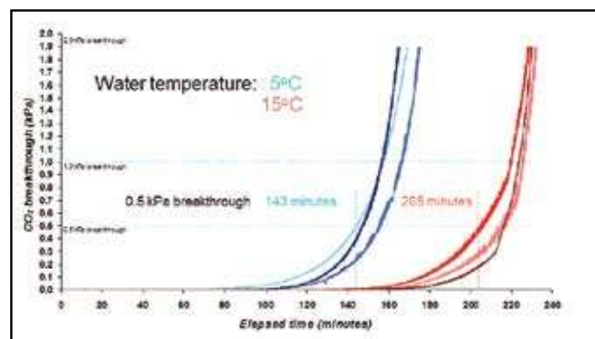
Figure 5. Reduction in absorbent canister endurance with a 10^\circ\text{C} ( 50^\circ\text{F} ) reduction in water temperature; n=3 runs at each temperature.
